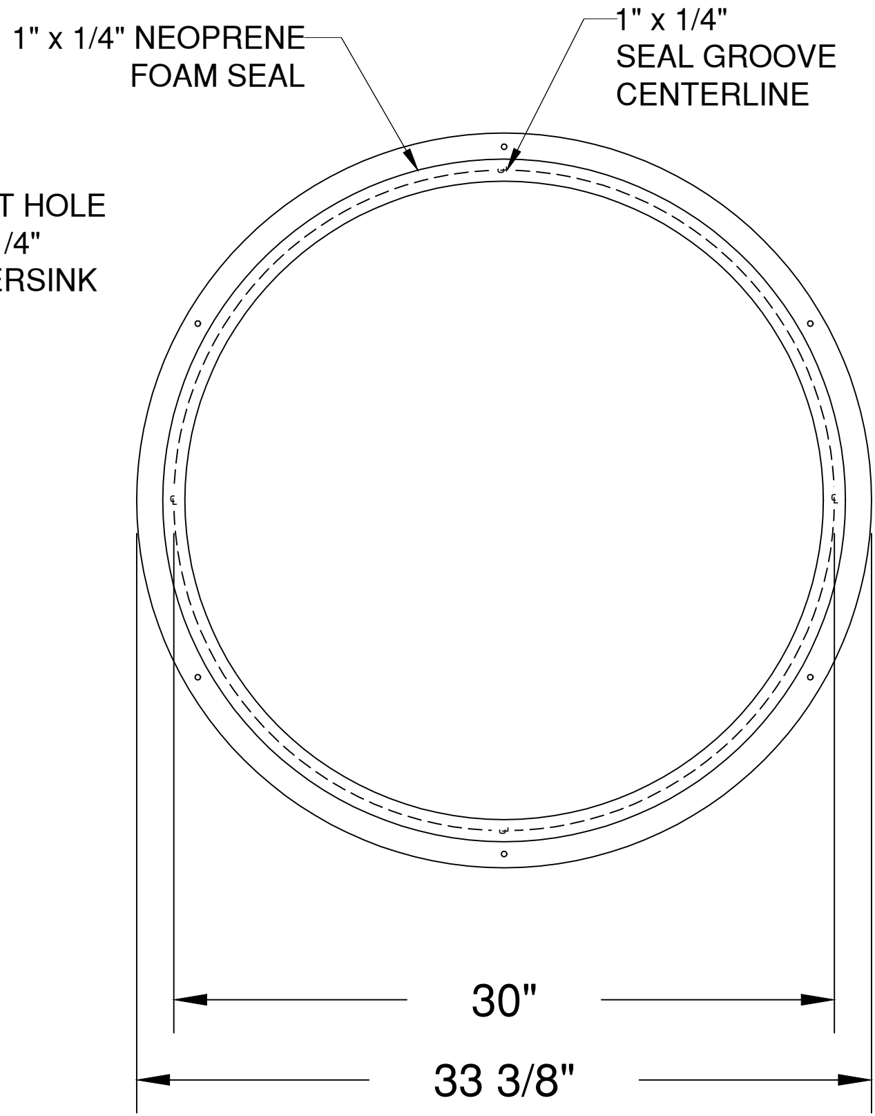
BOTTOM VIEW
