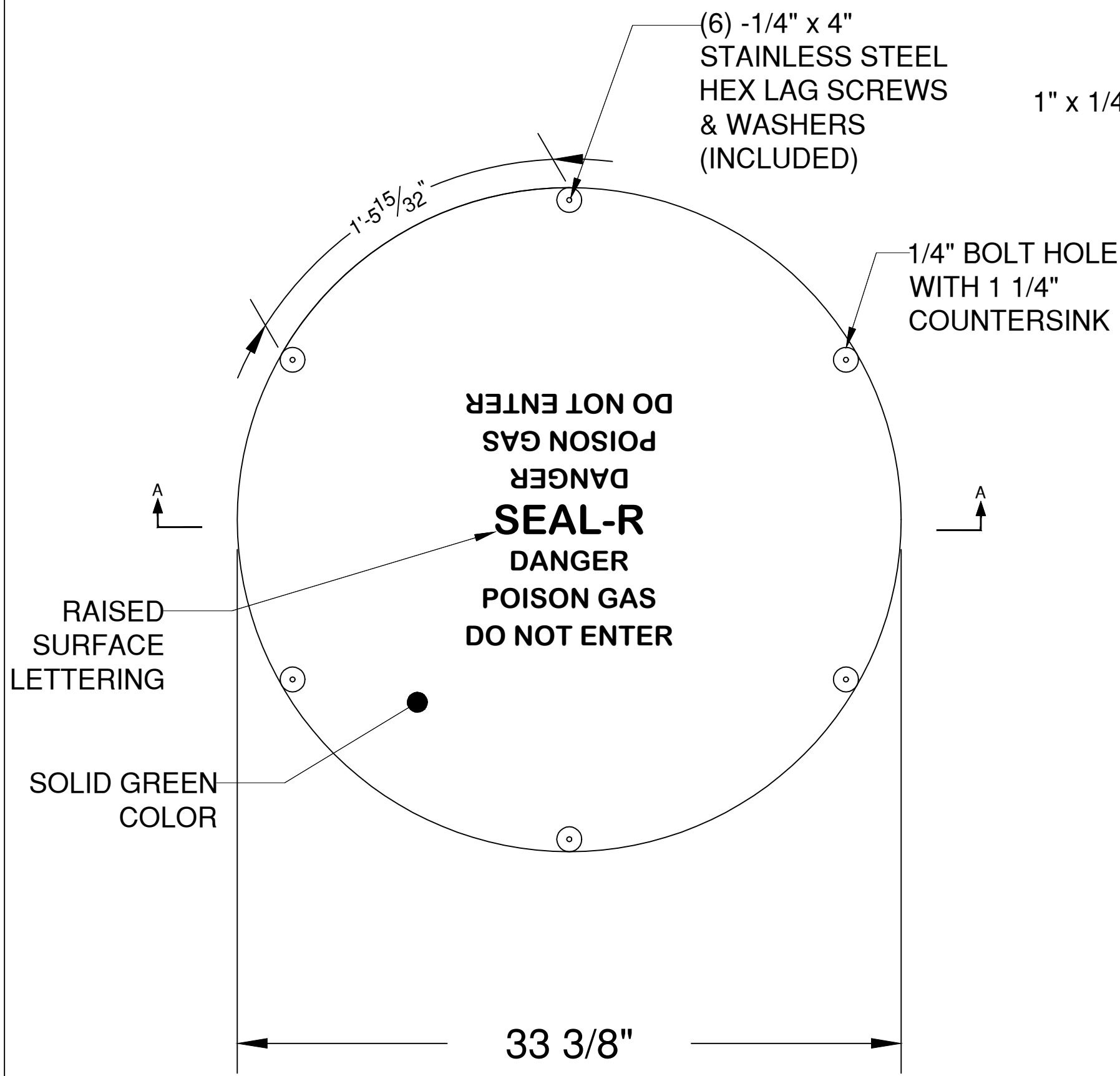
TOP VIEW
